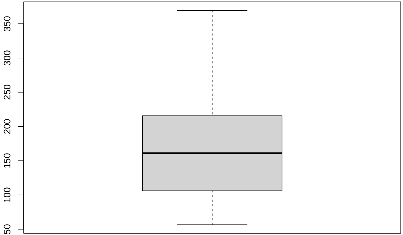
Boxplot – F
